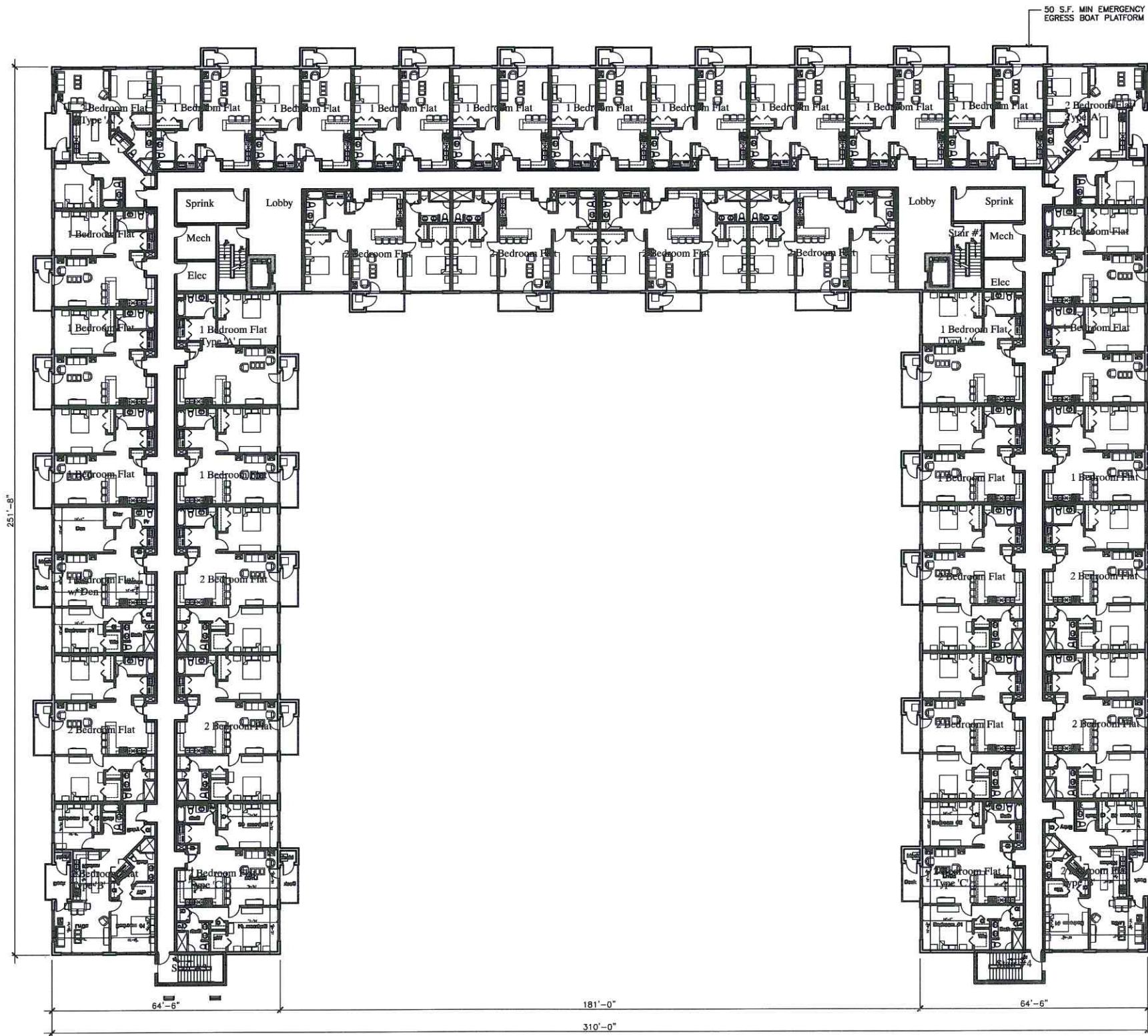
FIRST FLOOR PLAN SCALE 1/16" = 1'-0"
