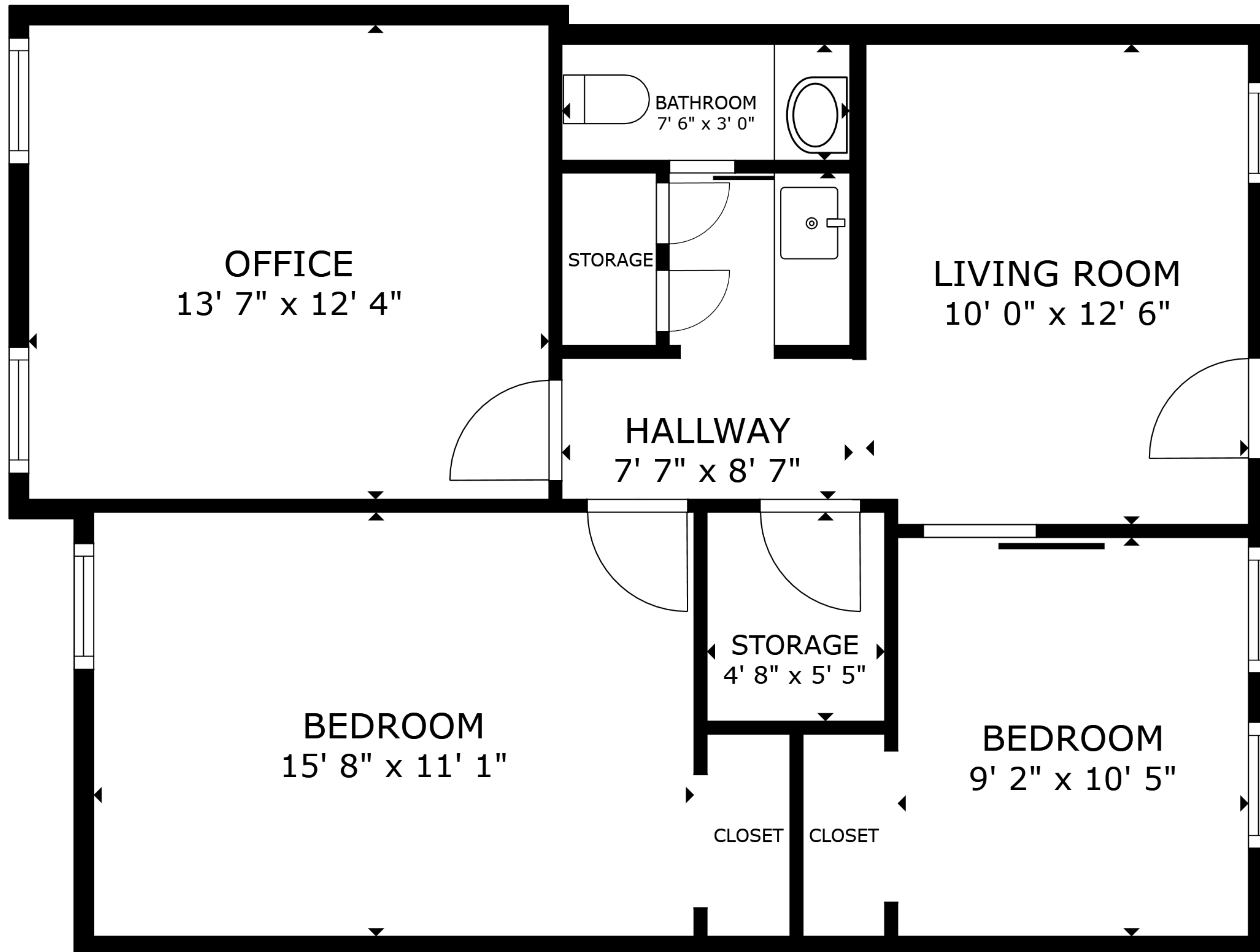
FLOOR PLAN
