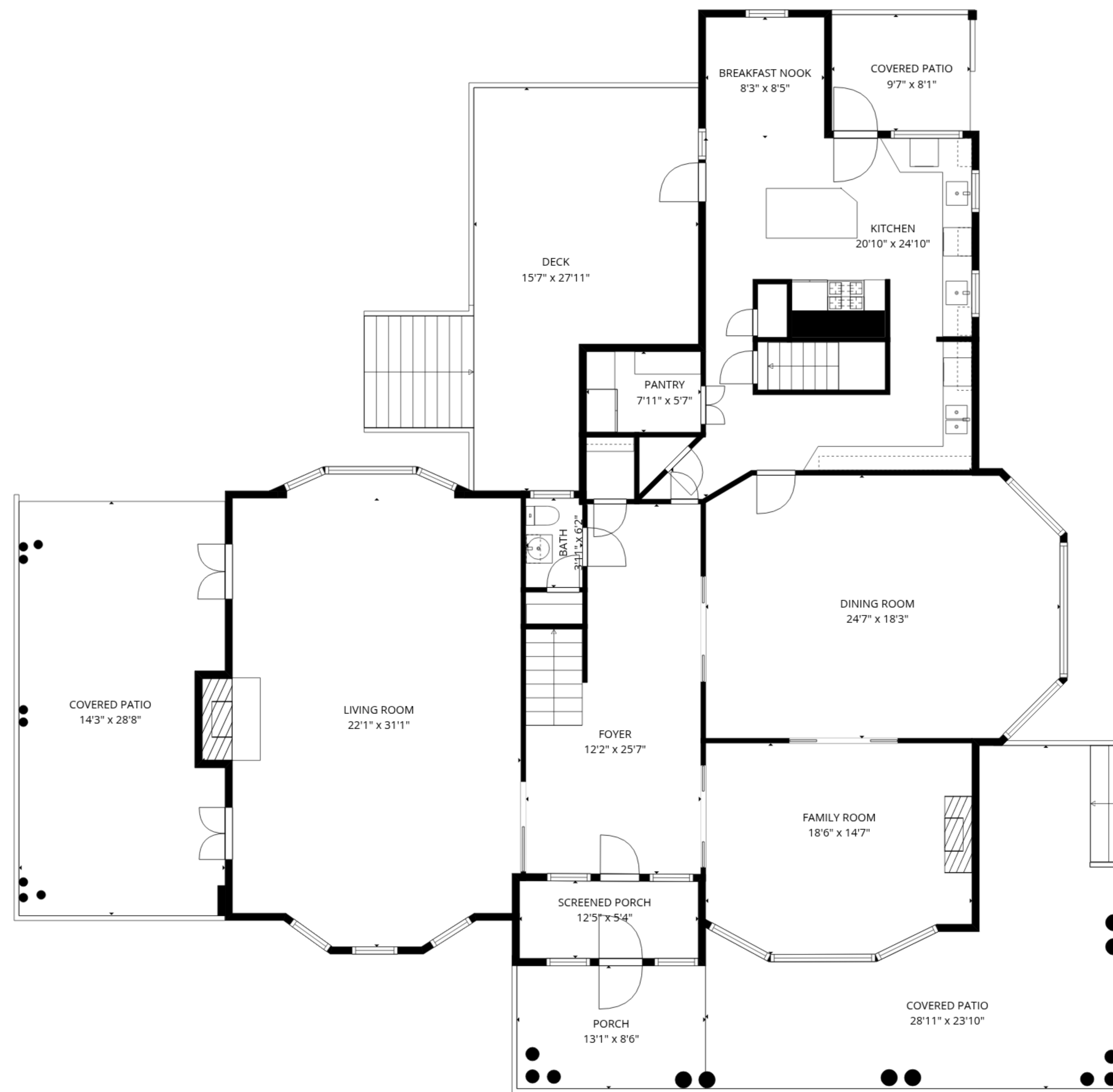
1st floor
