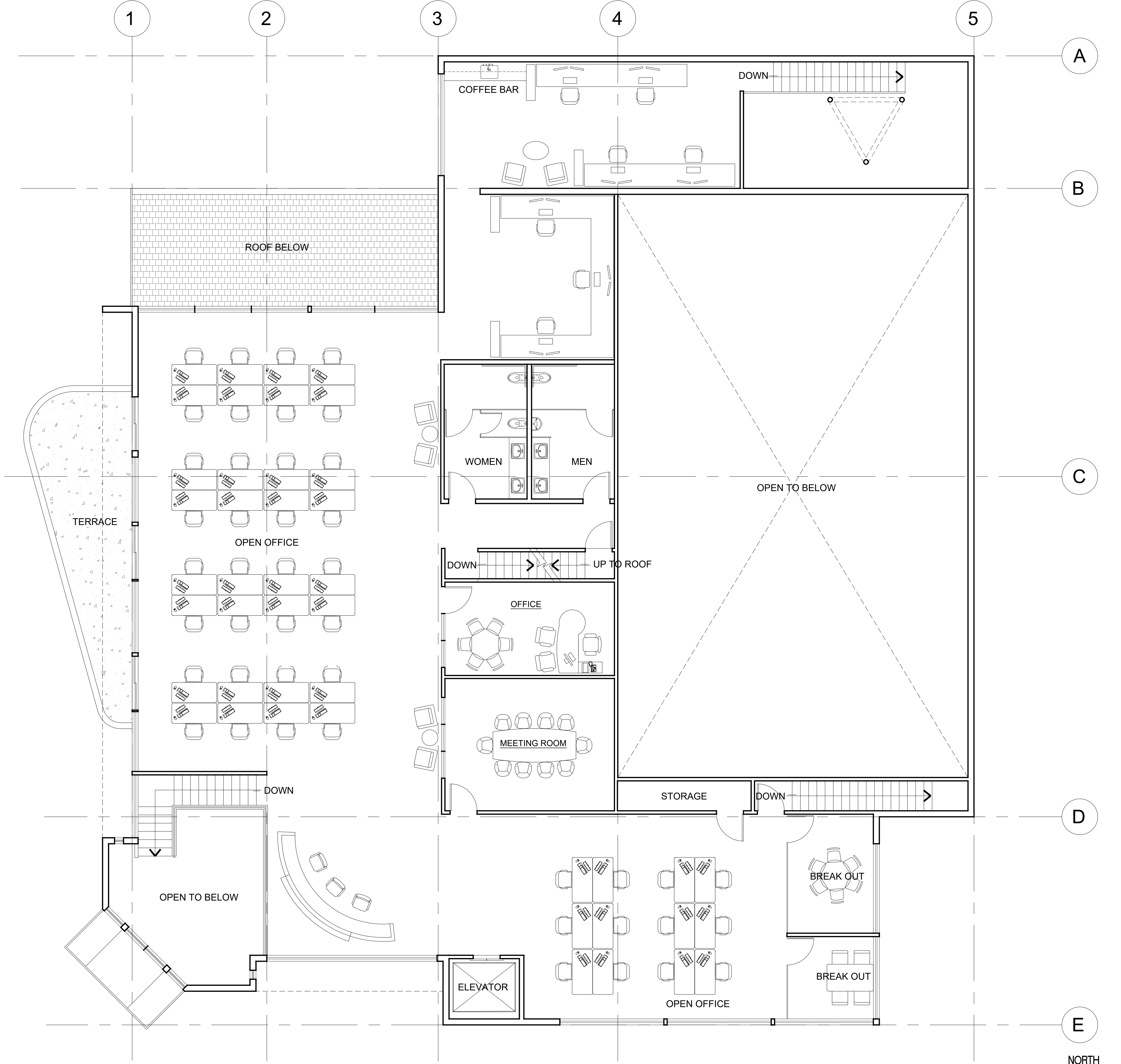
1 SECOND FLOOR PLAN SCALE: 3/16" = 1'-0"
