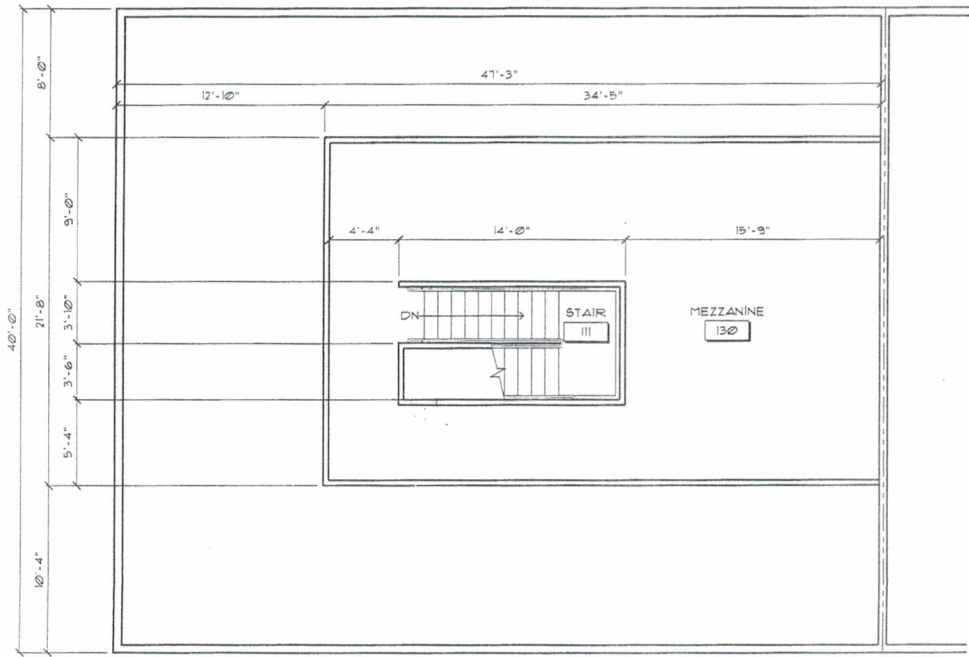
02 MEZZANINE PLAN SCALE: 3/16" = 1'-0"
