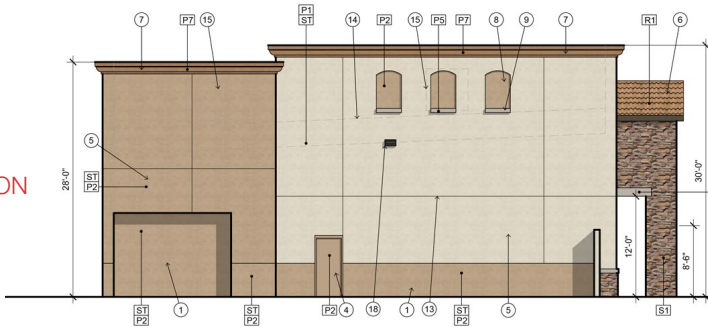
EAST ELEVATION
