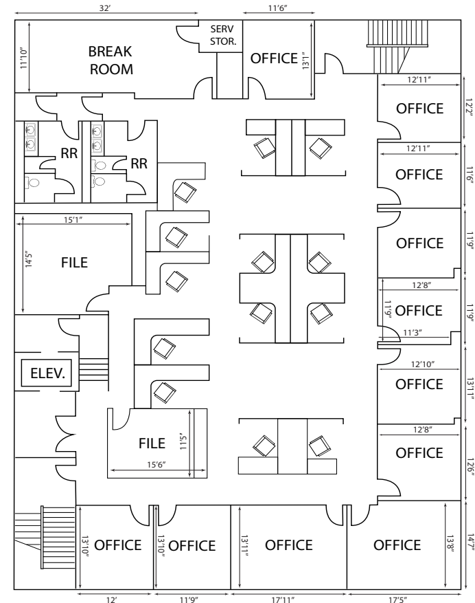
32'7" Column Spacing
