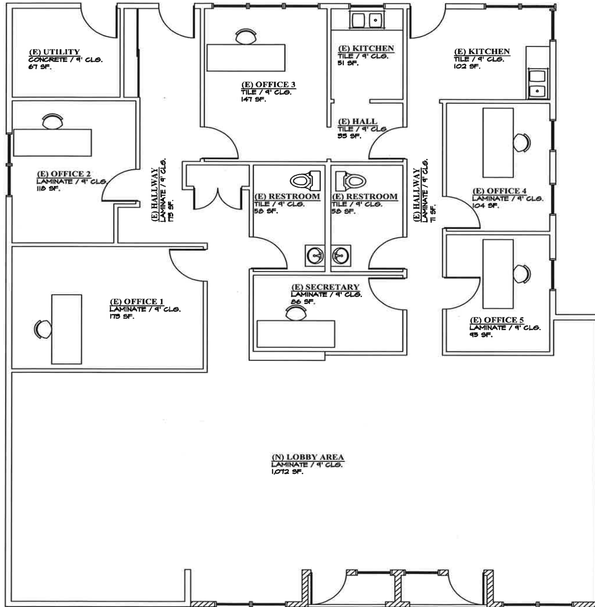
EXISTING FLOOR PLAN (2,893 S.F. TOTAL)
