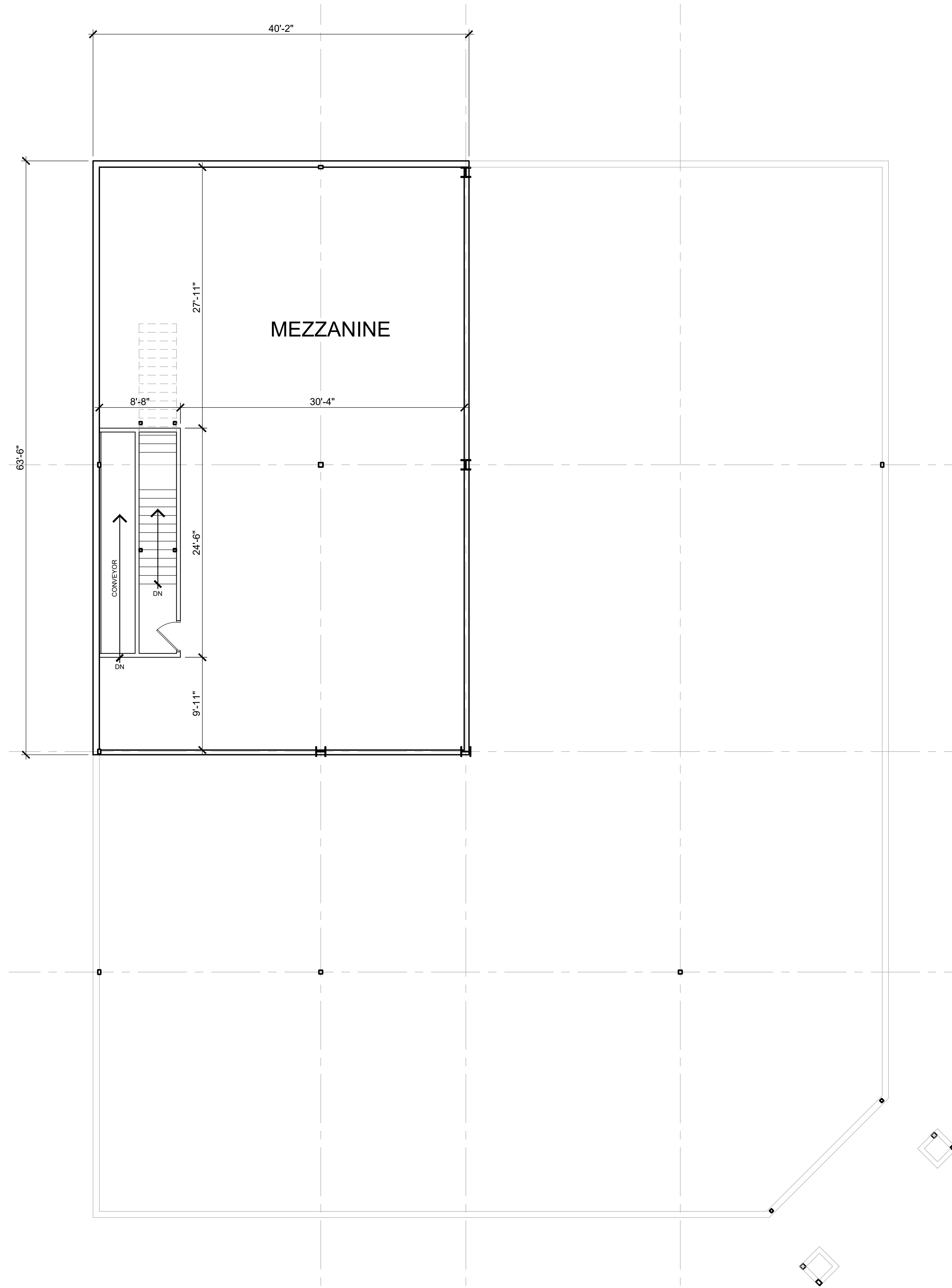
PROPOSED MEZZANINE PLAN
