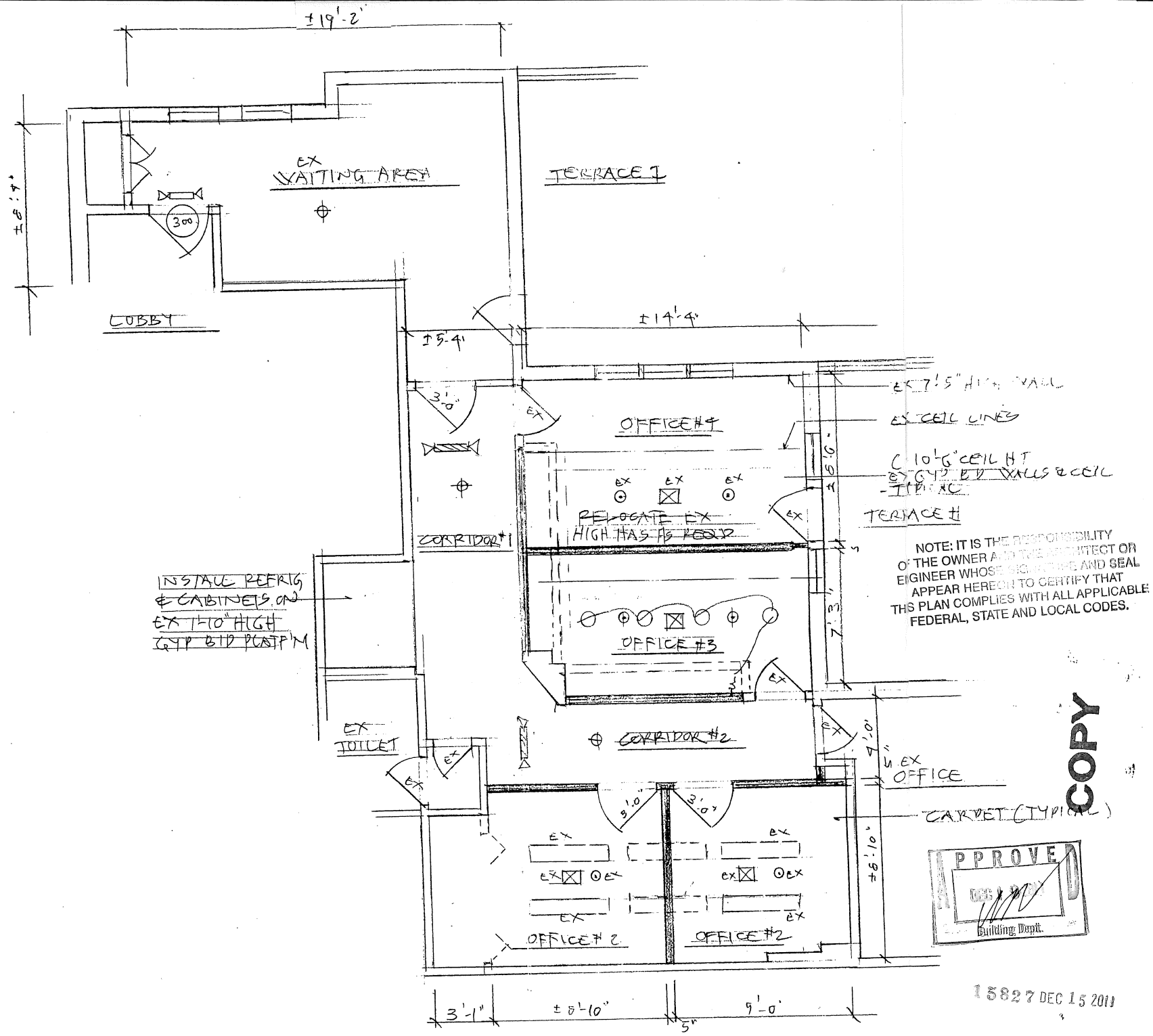
PARTIAL THIRD FLOOR PLAN scale: 1/4" = 1'-0"
