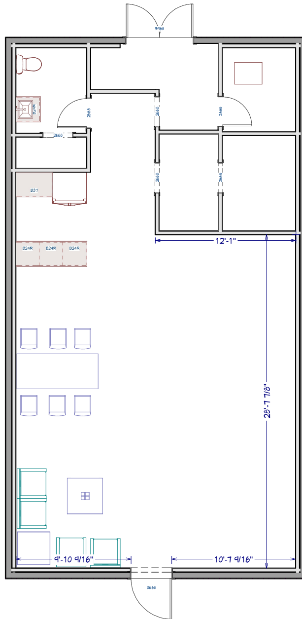
LIVING AREA 1195 SQ FT
