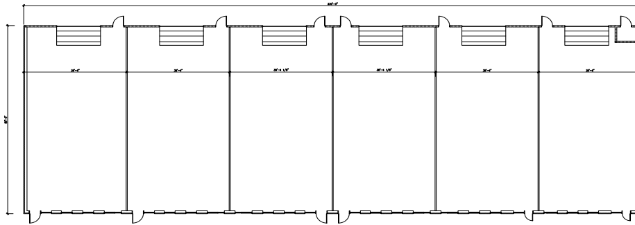
2 BUILDING 200 PRELIMINARY FLOOR PLAN SCALE: 3/16" = 1'-0"
