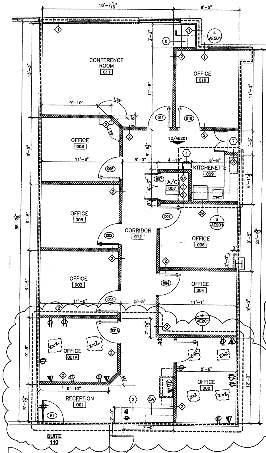
SUITE 110 FLOOR PLAN SCALE: 1/4" = 1'-0"
