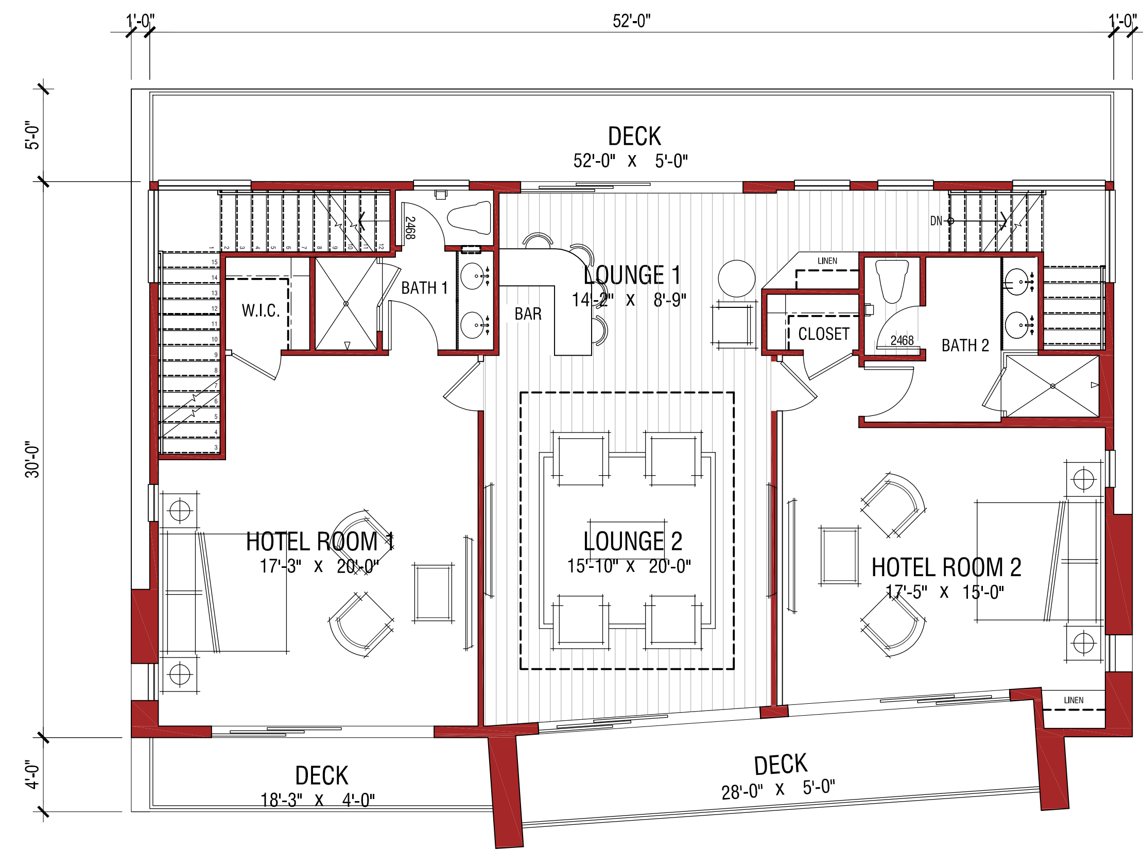
2ND FLOOR
