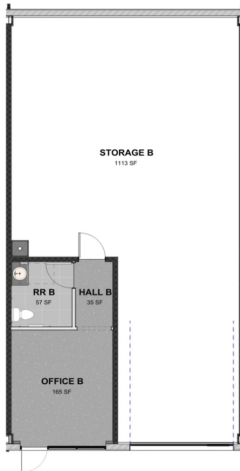
② FLOOR PLAN - LEASE - OFFICE TYPE B
