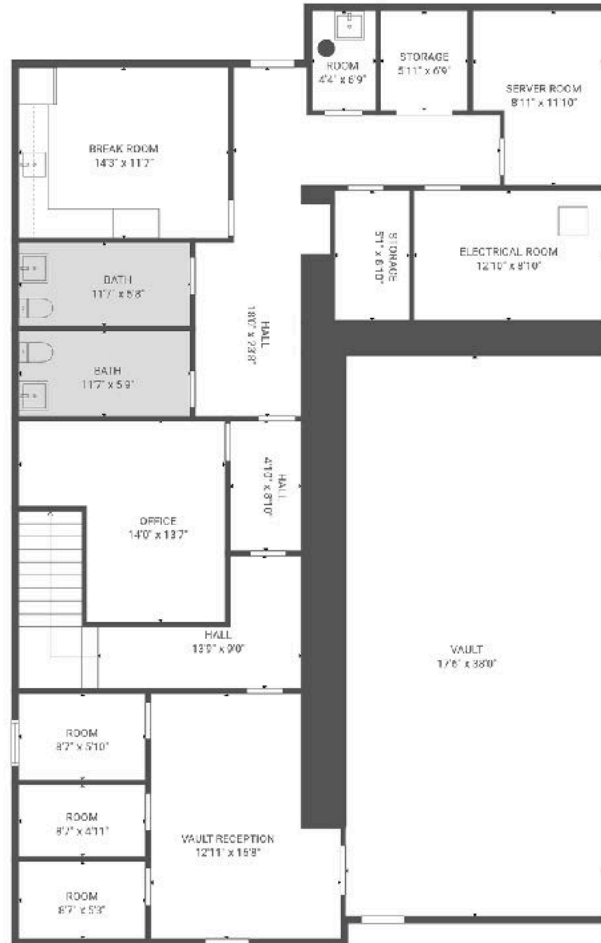
LOWER LEVEL
