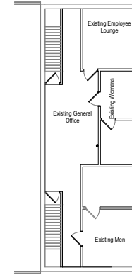
2 EXISTING 2nd FLOOR PLAN - NO WORK SCALE: 1/8" = 1'-0"
