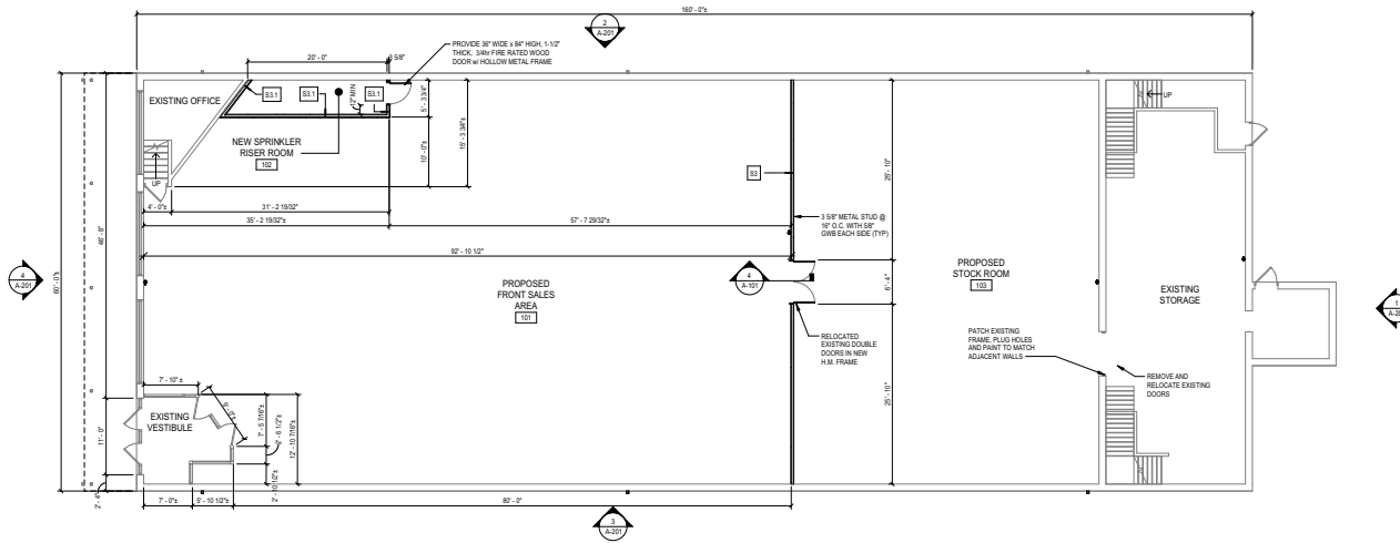
1 LEVEL 1 FLOOR PLAN SCALE: 1/8" = 1'-0"
