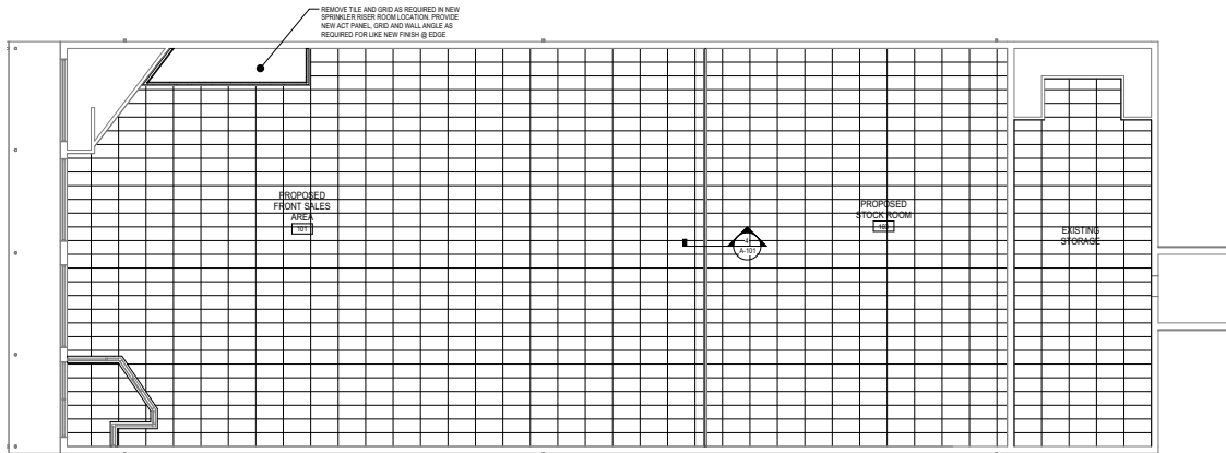
3 FIRST FLOOR REFLECTED CEILING PLAN SCALE: 1/8" = 1'-0"
