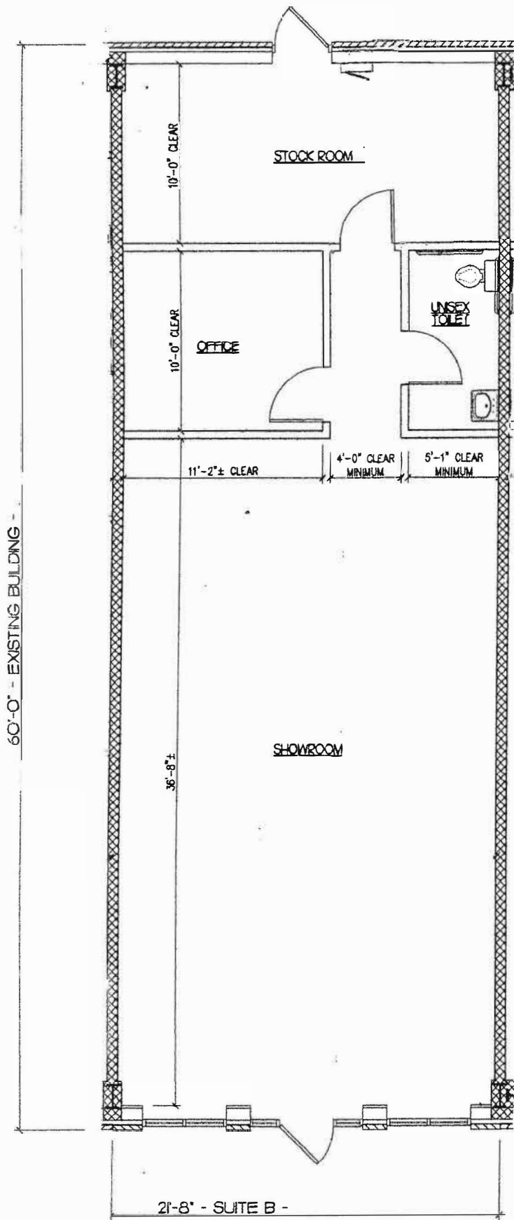
UPFIT FLOOR PLAN
