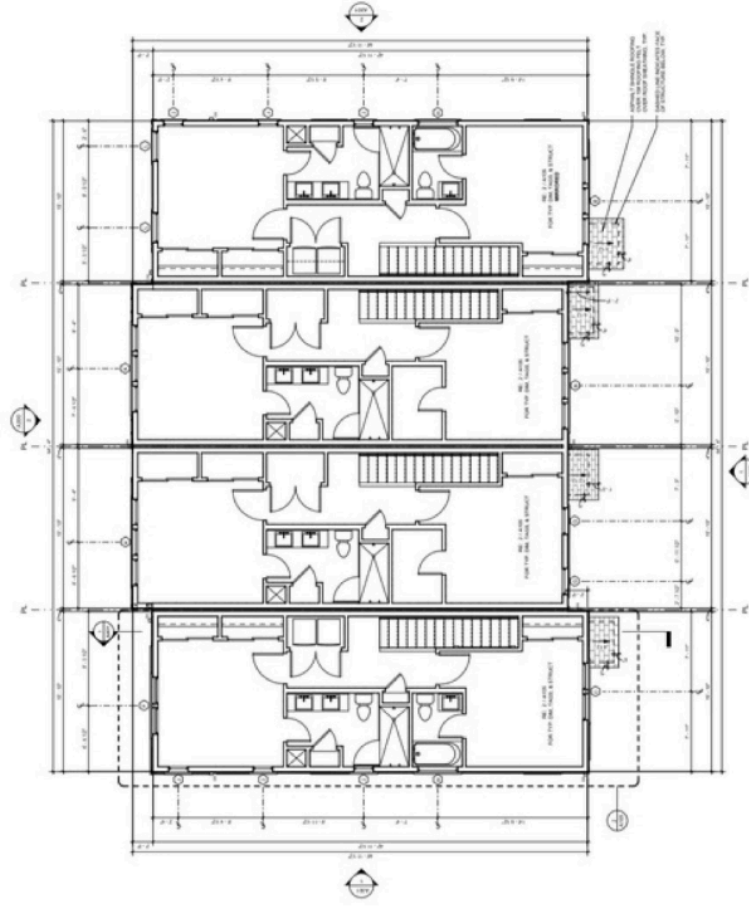
1 2ND FLOOR 1/4" = 1'-0"
