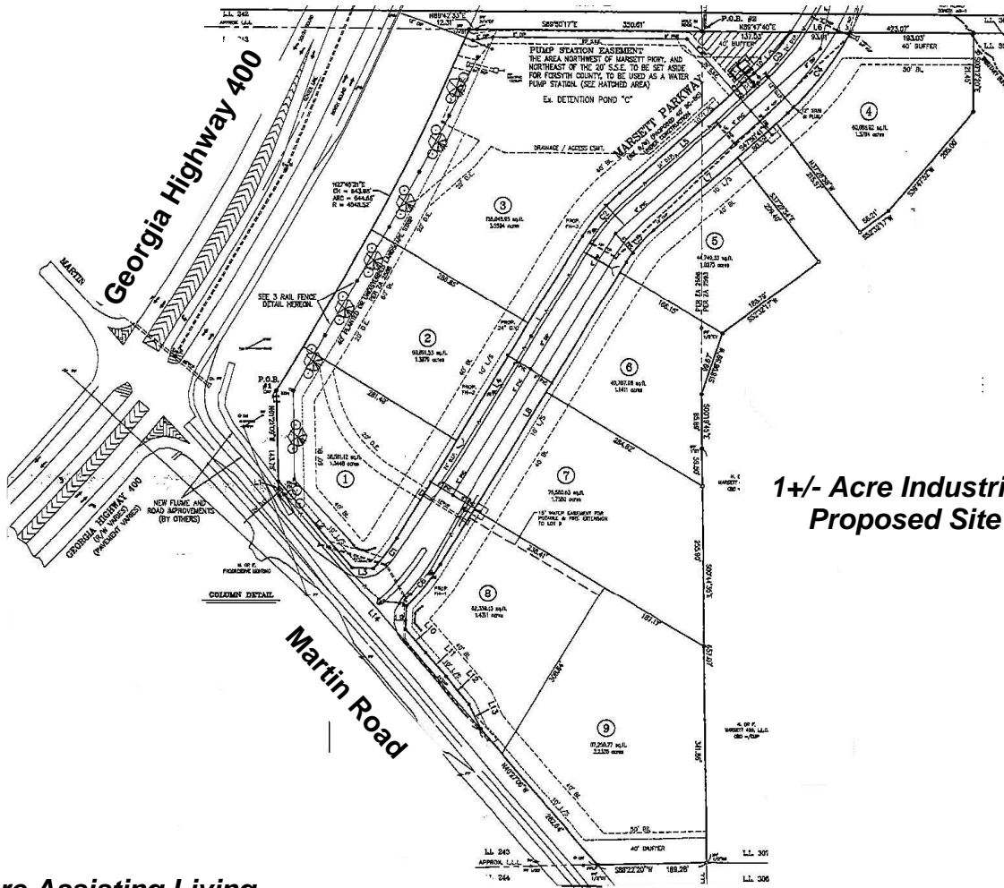
26+/- Acre Assisting Living Proposed Site plan
