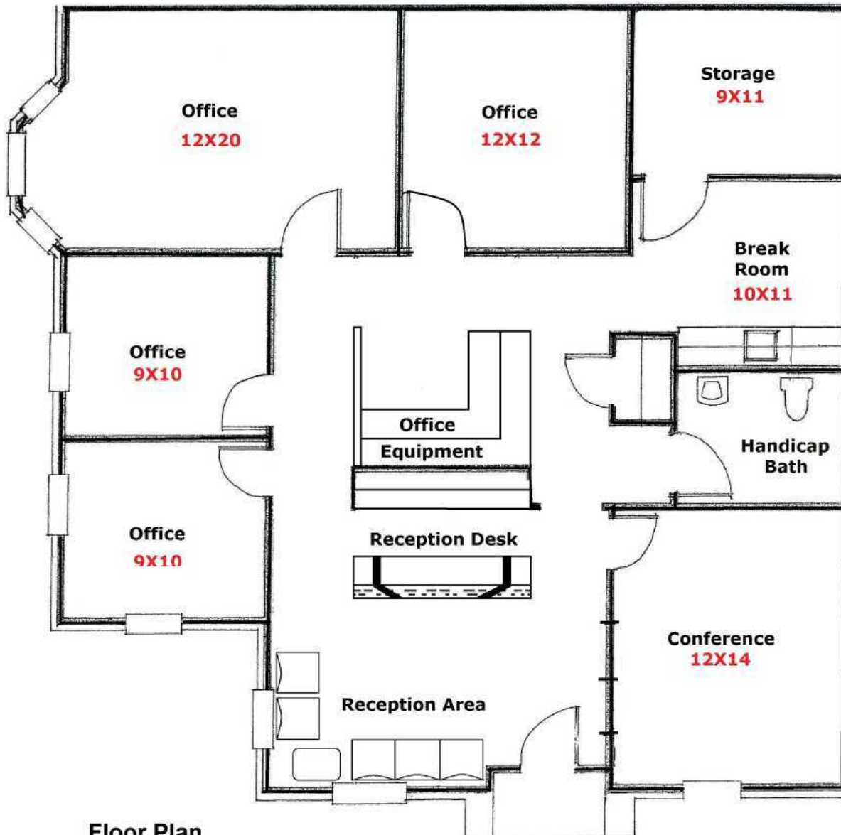
Floor Plan 1700sf +/-
