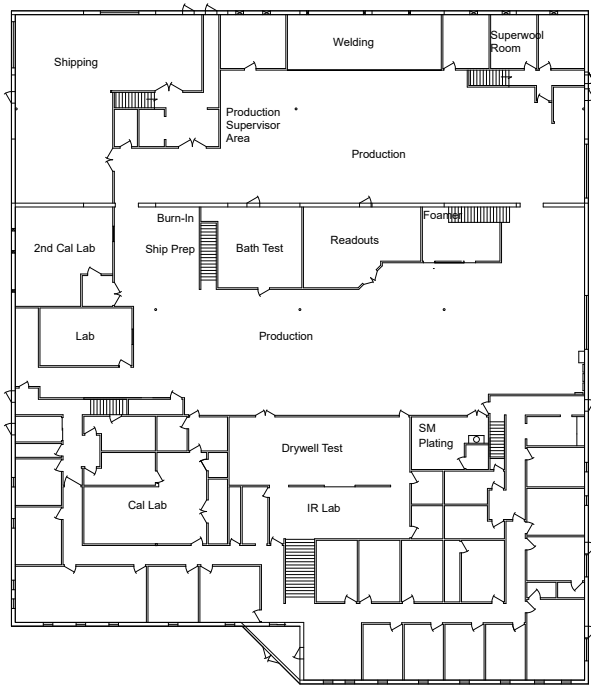
1st Floor
