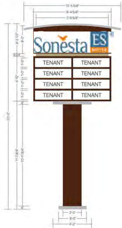
GRAPHIC DETAIL SCALE: 1/4" = 1'-0"
