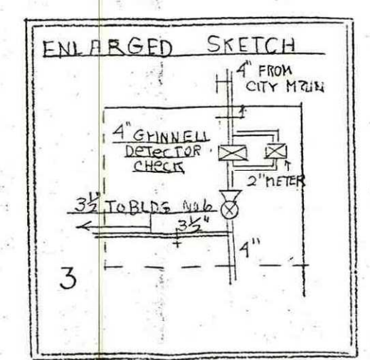
SECTION 4-E'
