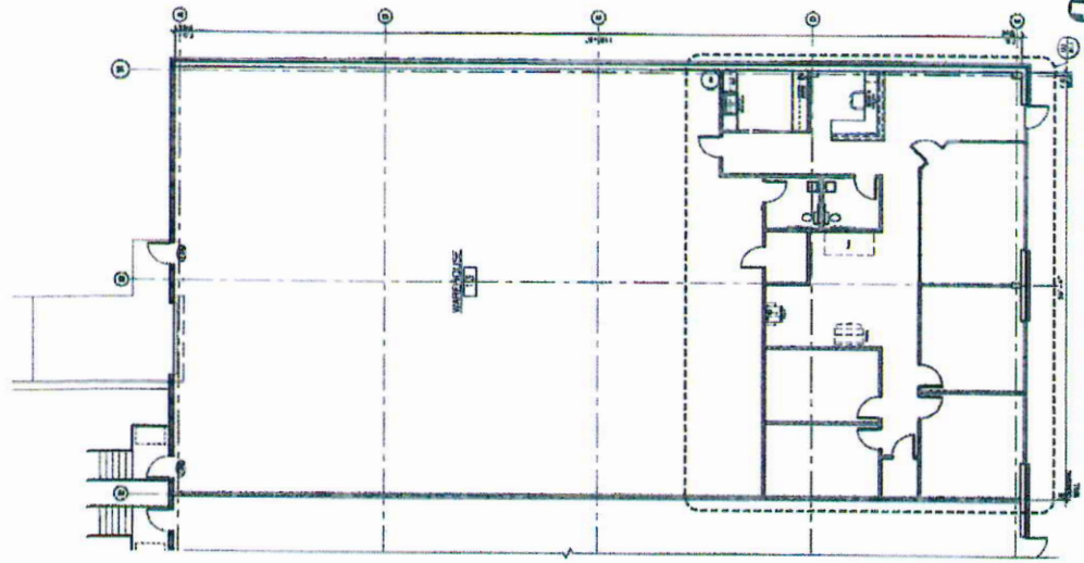
01 FLOOR PLAN: Rev (1/2" = 1'-0")
