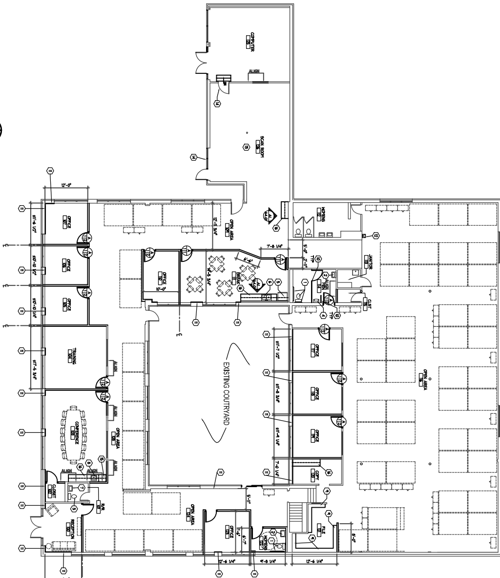
A1 FLOOR PLAN - 1st floor
