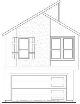
ELEVATION C
