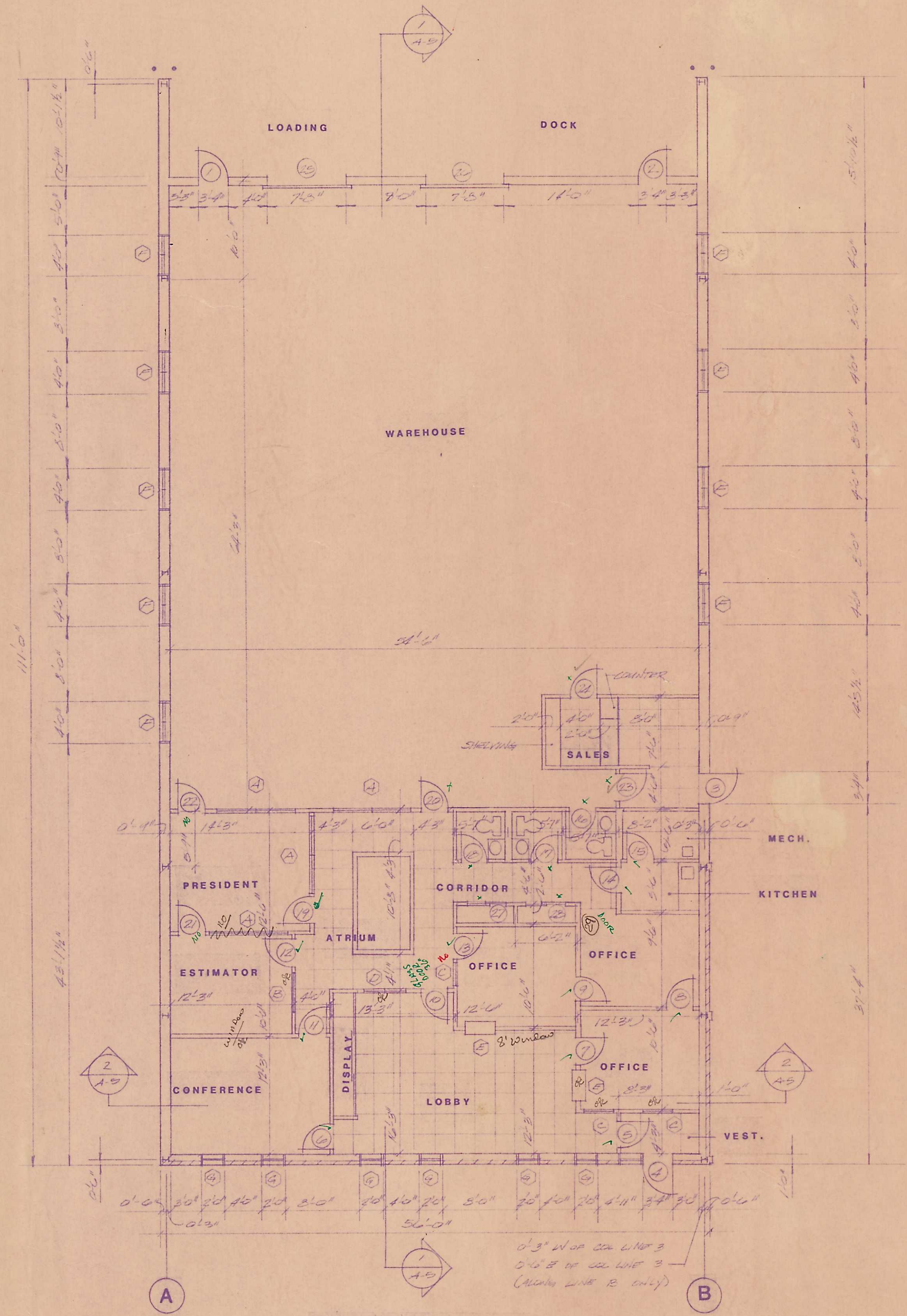
FLOOR PLAN
