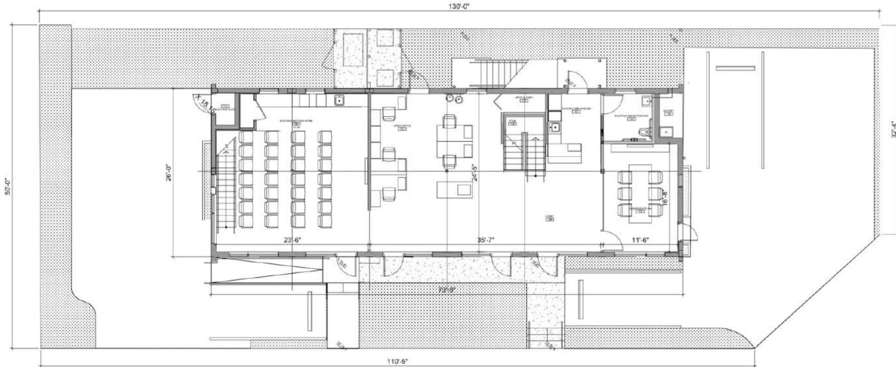
1 GROUND FLOOR AS BUILT PLAN SCALE: 3/8" = 1'-0"
