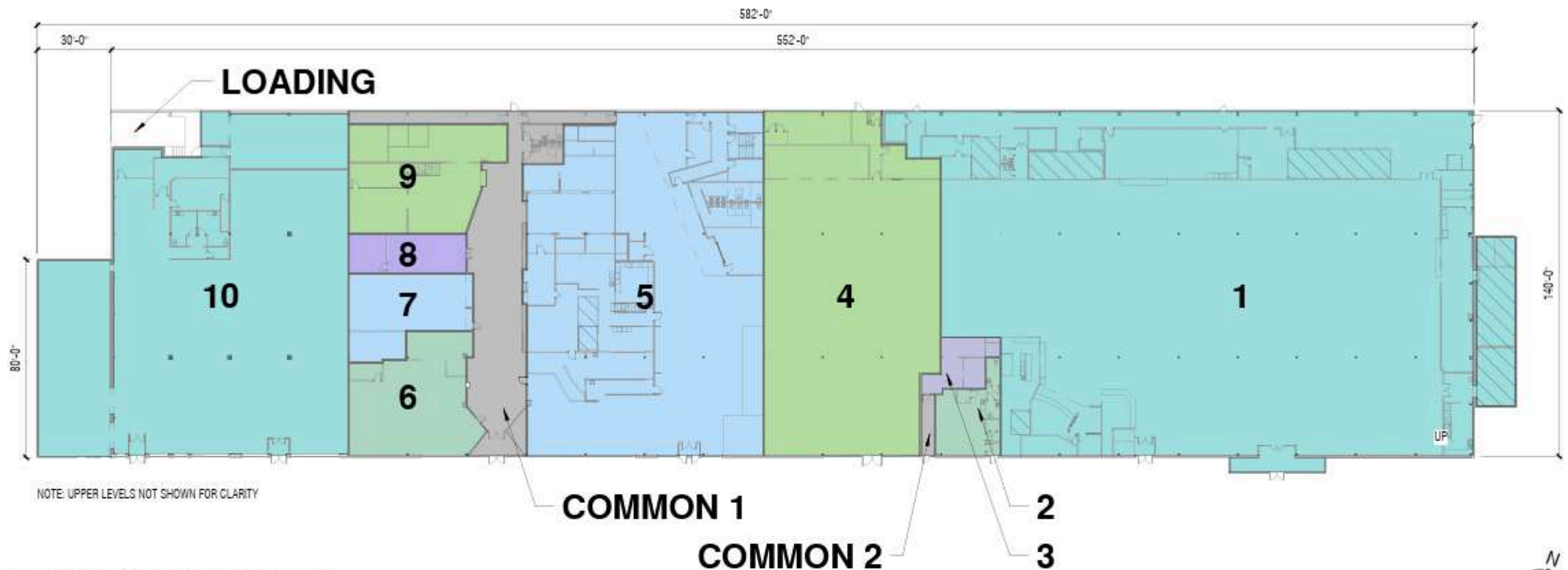
TENANT SPACE LAYOUT PLAN 1" = 40'-0"
