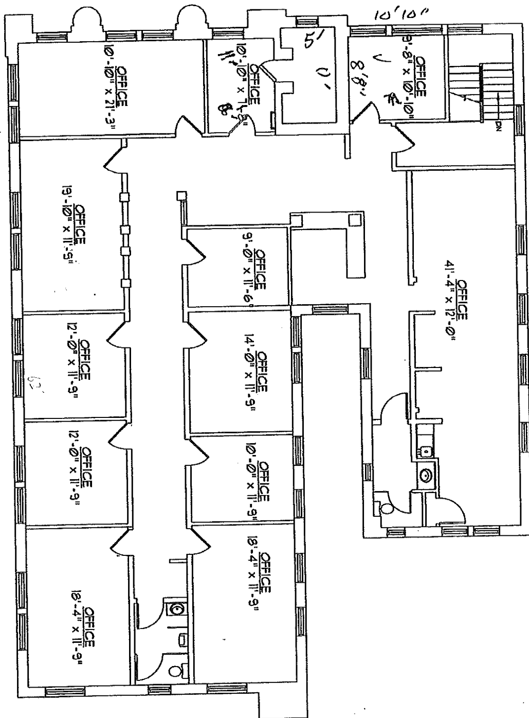
1 SECOND LEVEL PLAN SCALE: 3/32" = 1'-0"
