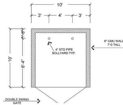
DUMPSTER PAD DETAIL
