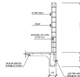
DUMPSTER WALL SECTION
