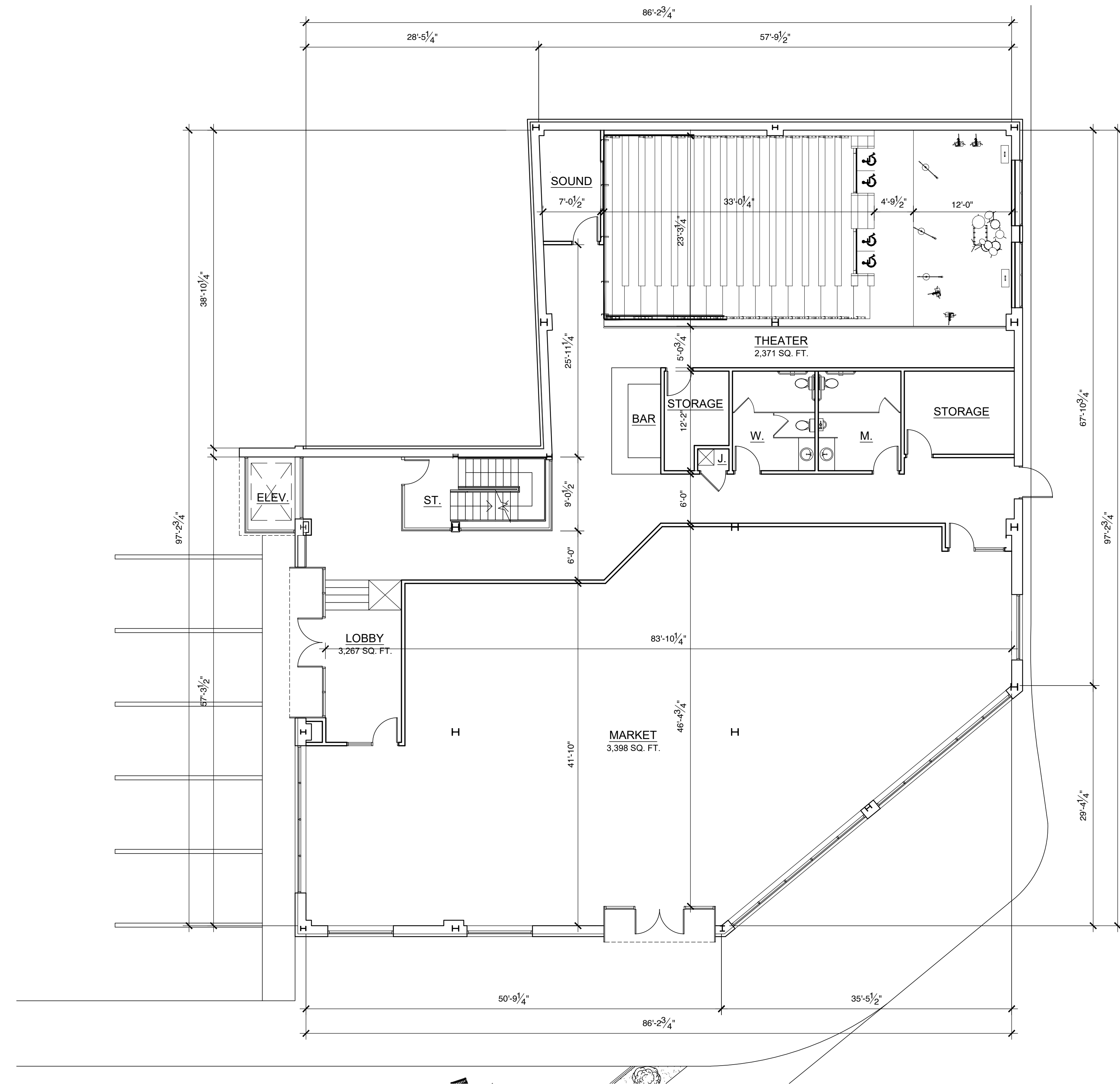
FIRST LEVEL PLAN SCALE: 1/8"=1'-0"
