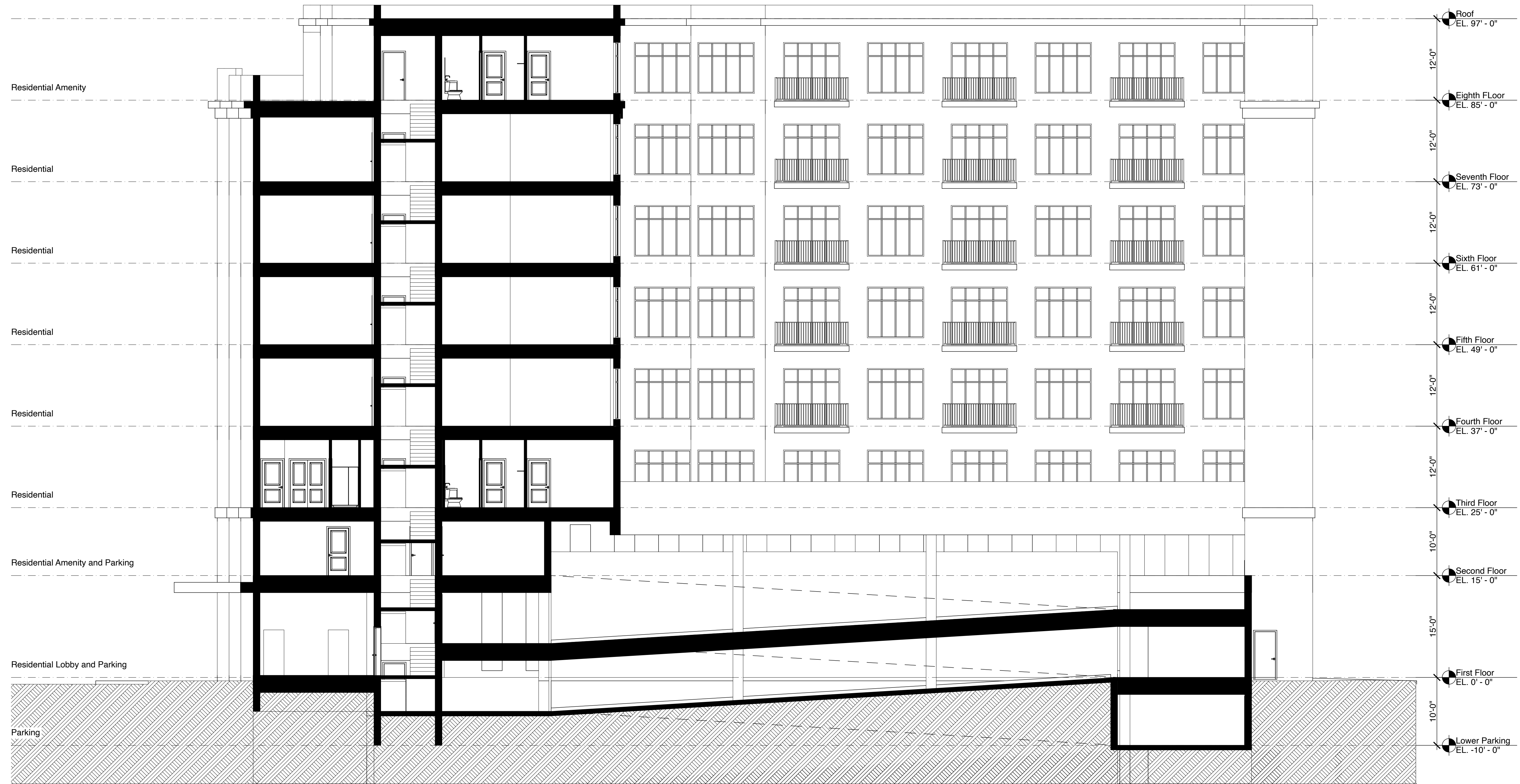
SECTION
