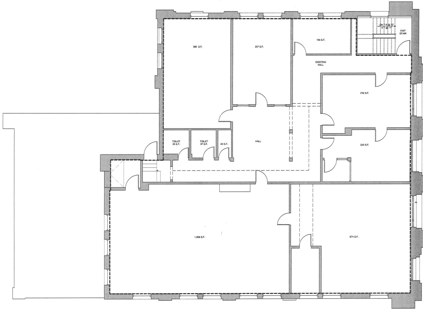
LEVEL 2B FLOOR PLAN TOTAL FLOOR AREA = 3,900 G.S.F. AVAILABLE AREA = 3,793 G.S.F.
