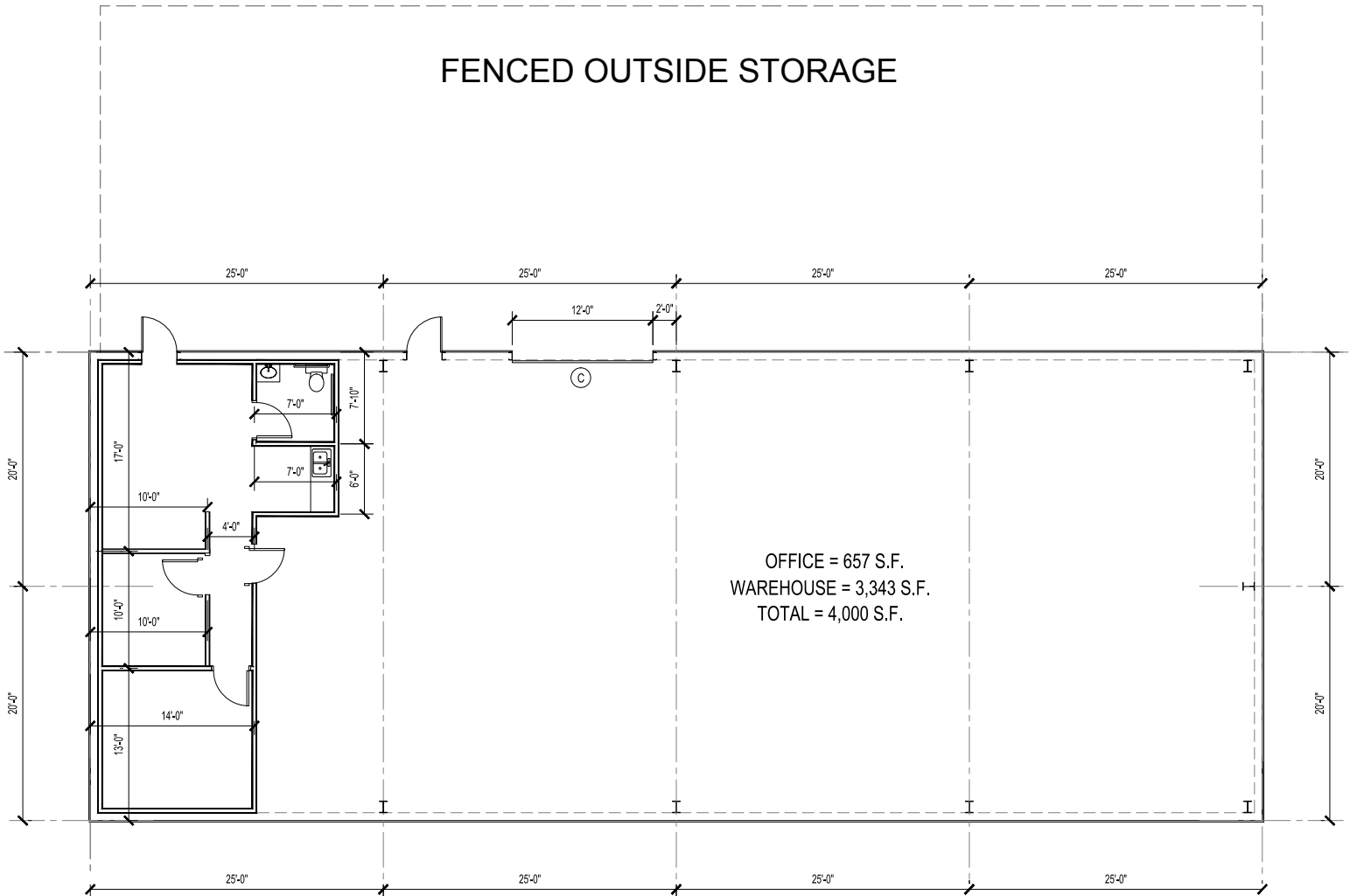
FLOOR PLAN 3/16"=1'-0"
