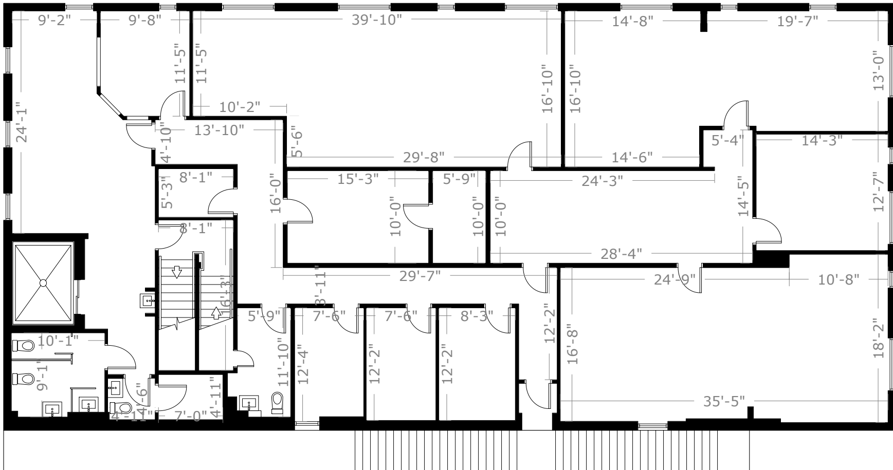
2nd Floor, 912 Central Ave | 3/32" = 1'-0"
