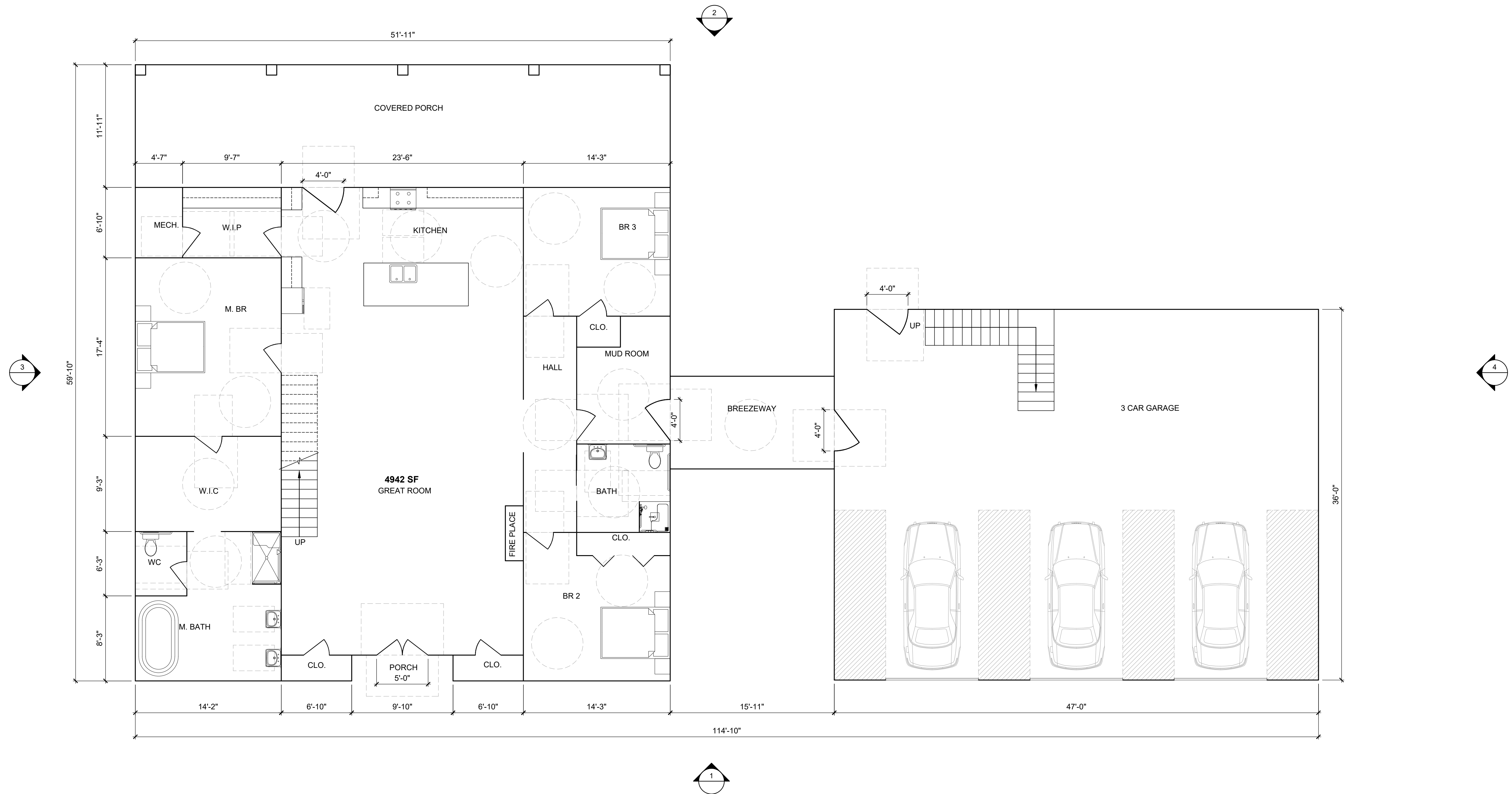
1 ENLARGED 501 FLOOR PLAN 3/16" = 1'-0"
