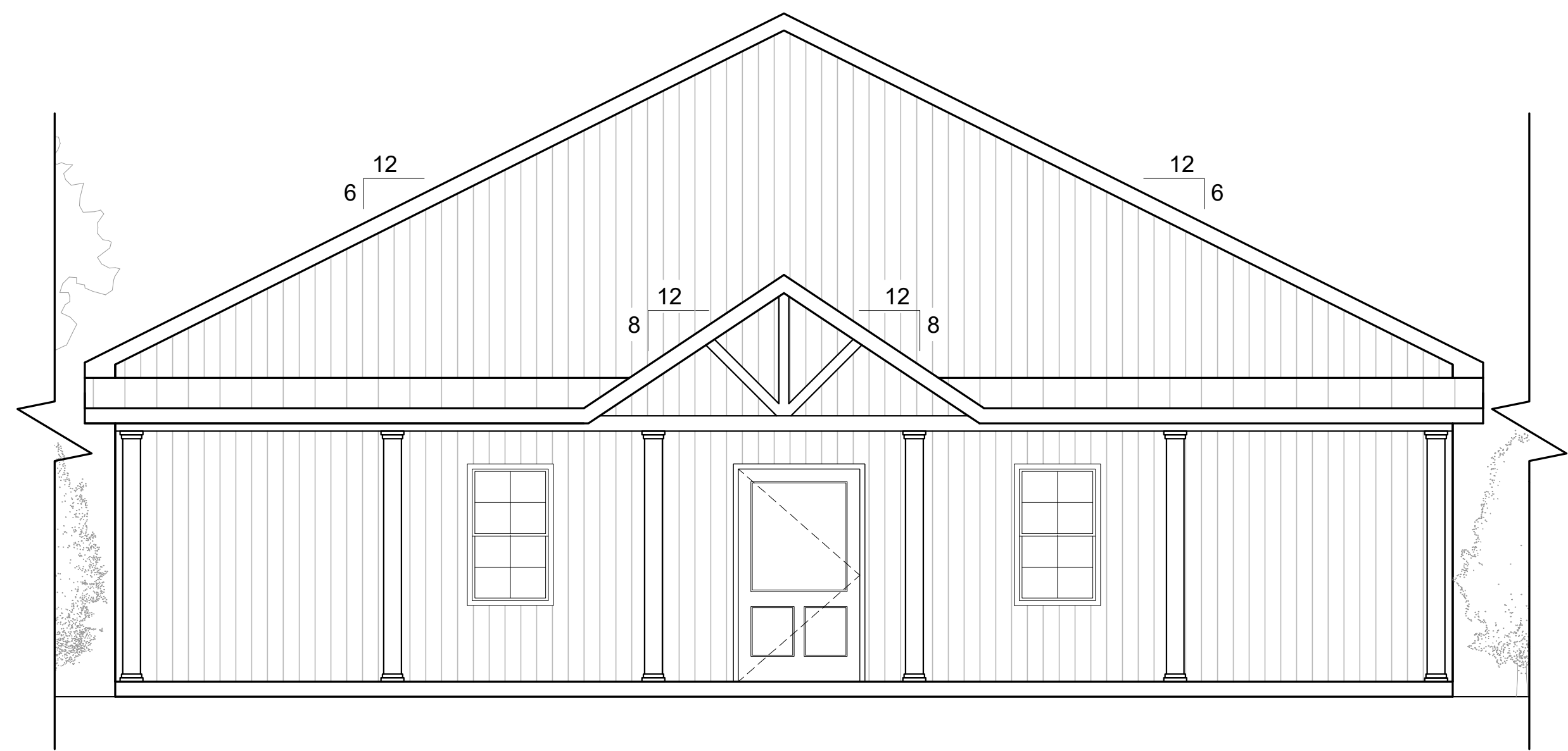
2 ELEVATION 518, 532, 550, 566, 586 3/16" = 1'-0"
