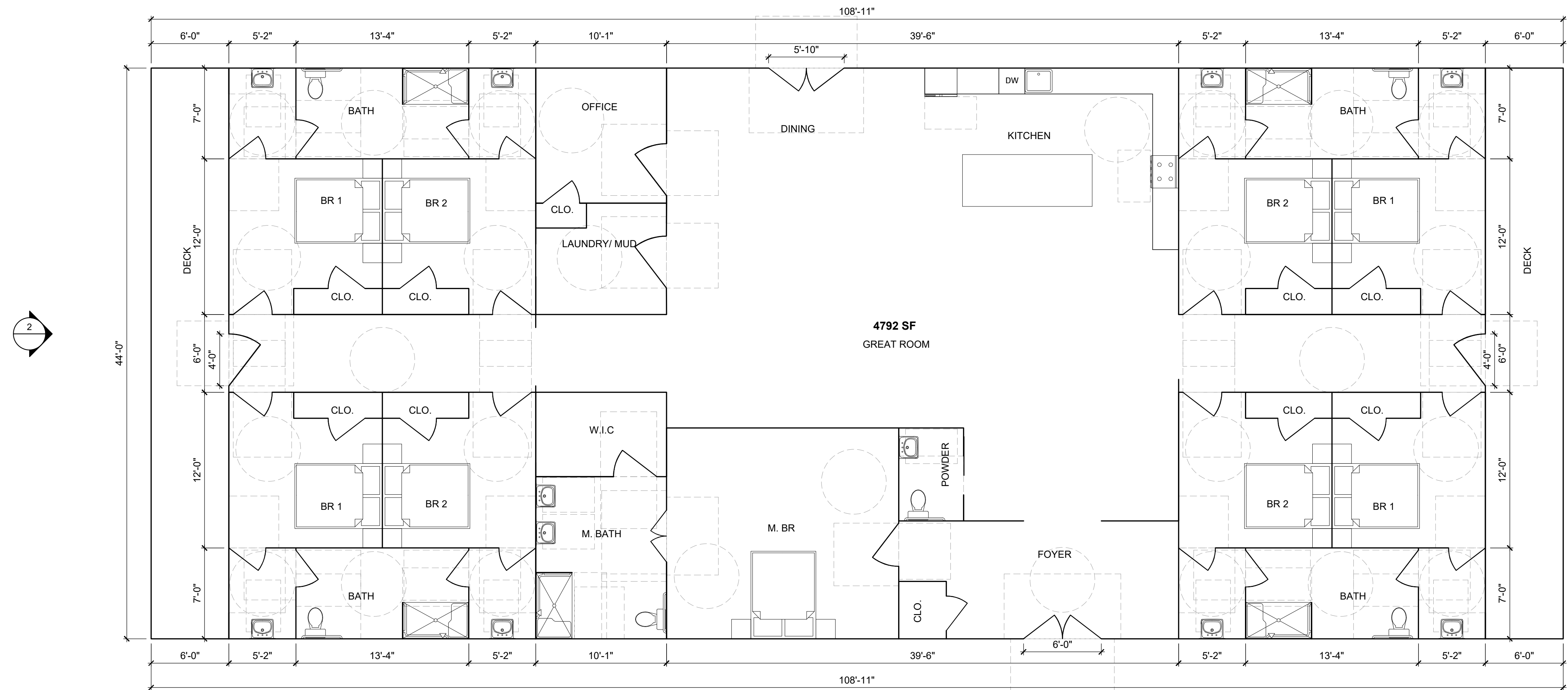
1 ENLARGED 518, 532, 550, 566, 586 FLOOR PLAN 3/16" = 1'-0"
