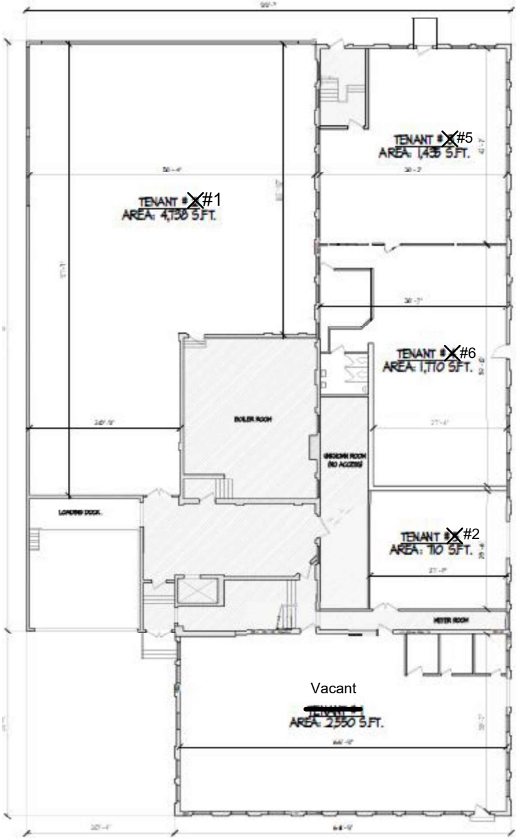
EXISTING FIRST FLOOR PLAN SCALE: 3/32" = 1'-0" BLDG. GROSS AREA: 5,280 SQ. FT.
