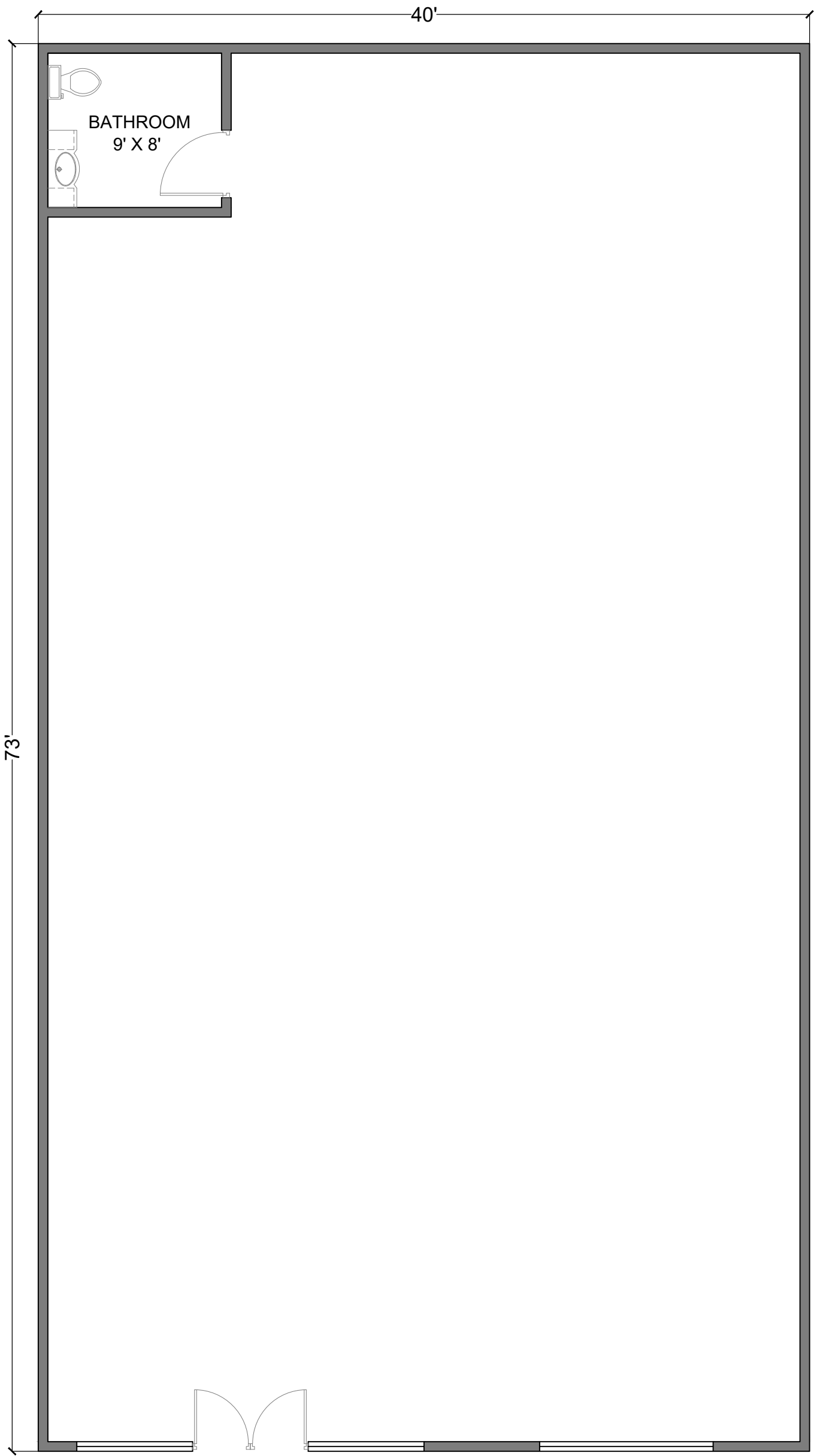
FLOOR PLAN
