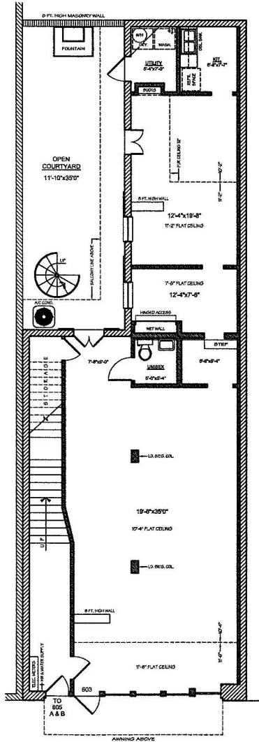
603/605 JULIA STREET - NEW ORLEANS FIRST FLOOR LAYOUT
