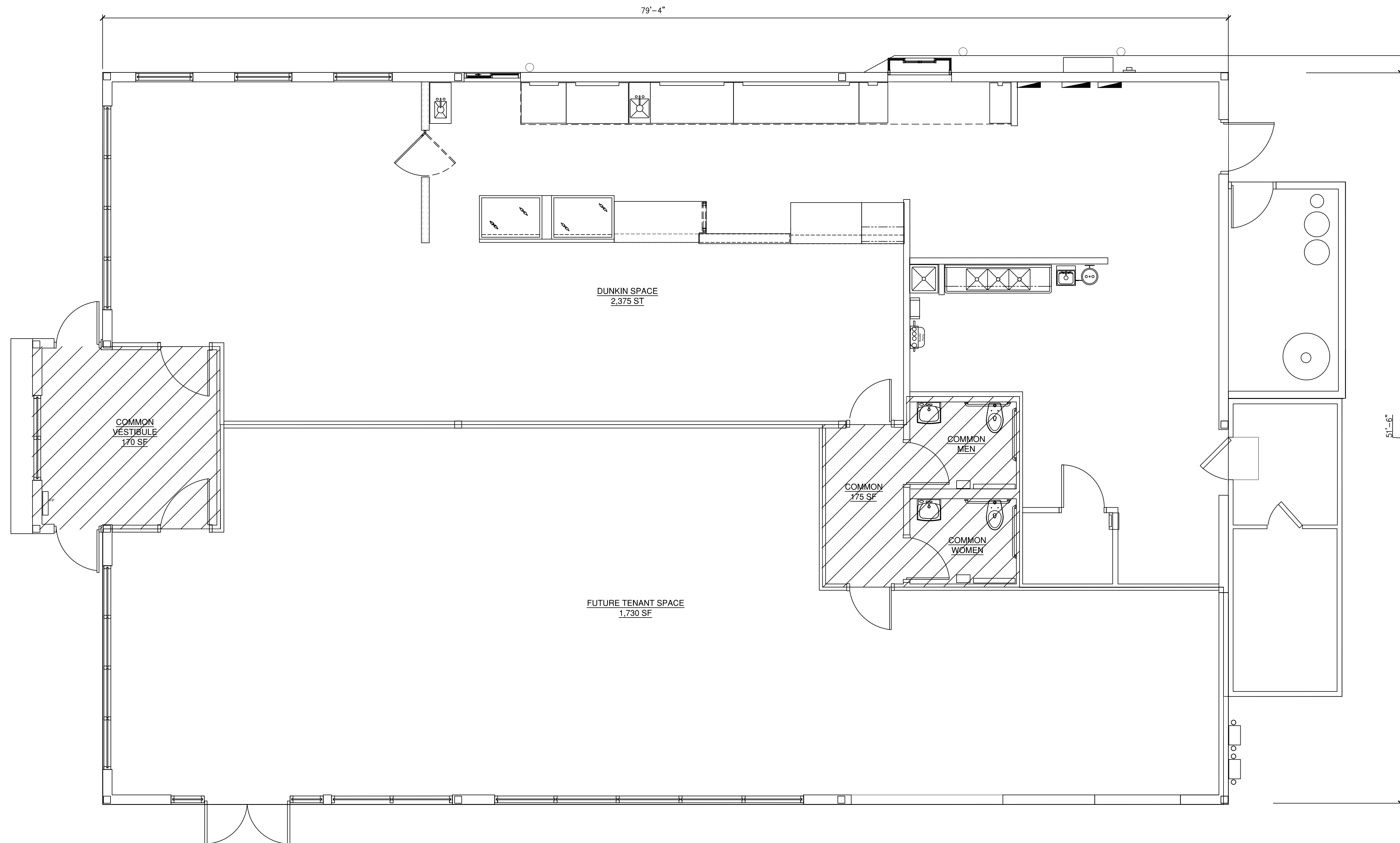
1 FLOOR PLAN 1/4" = 1'-0"
