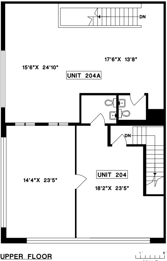
UPPER FLOOR
