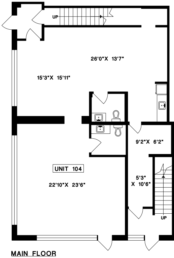
MAIN FLOOR
