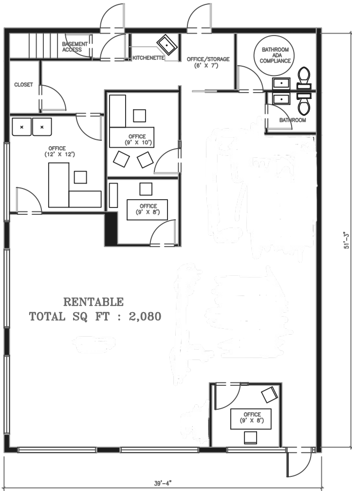
FIRST FLOOR
