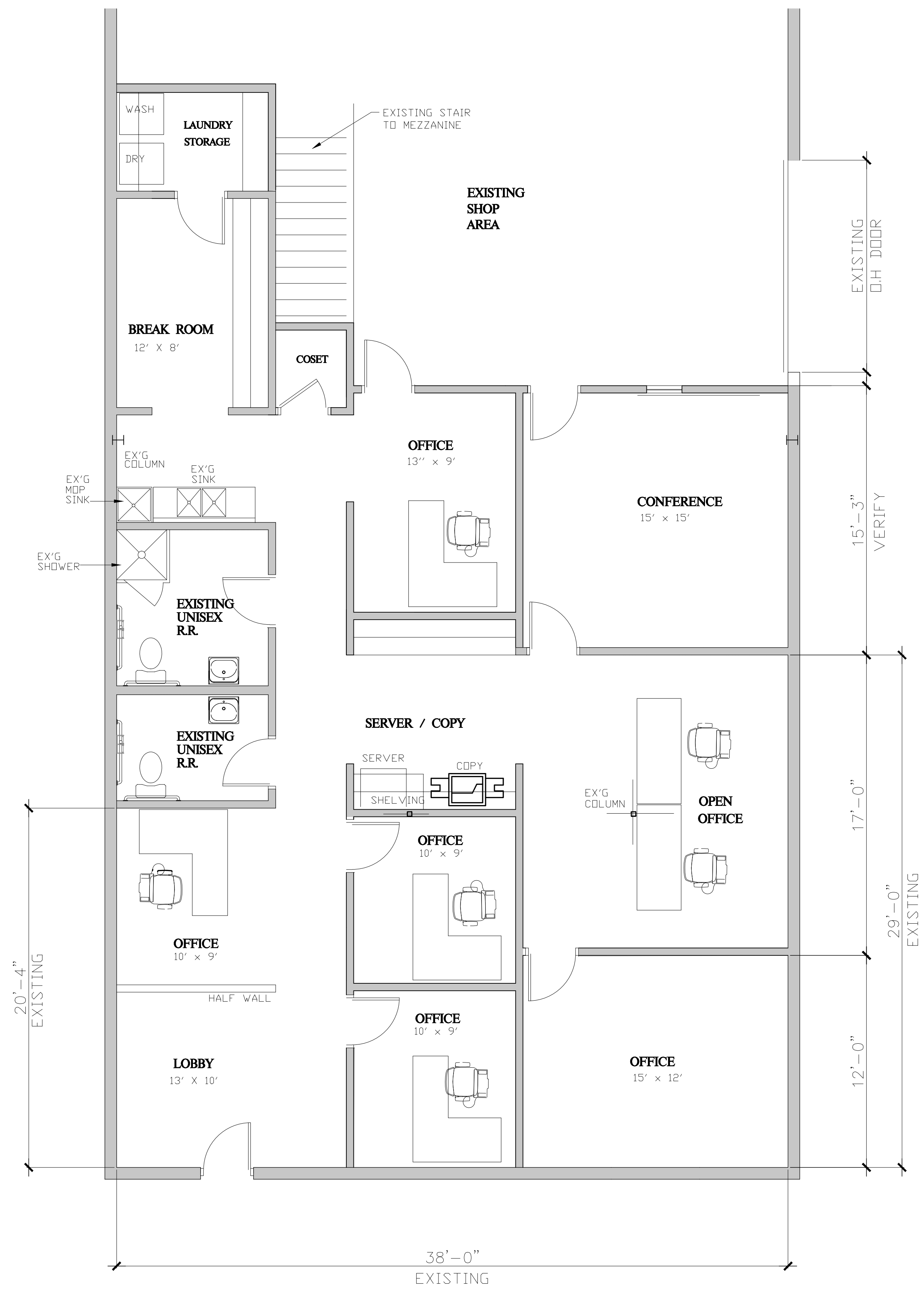
FLOOR PLAN 1,946 SF APPROX. GROSS SQ FT 0' 4' 8' 16' NORTH
