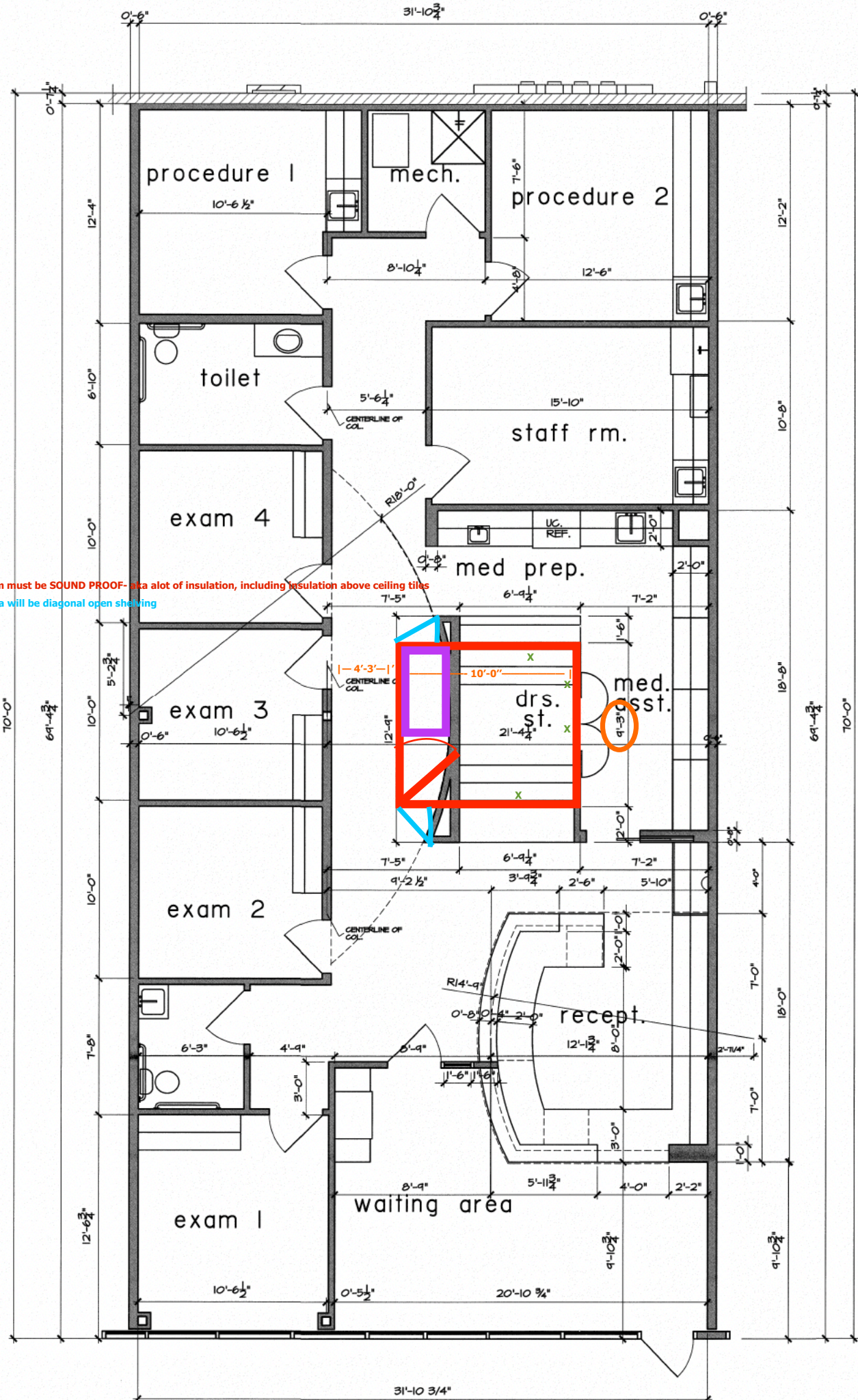
dimensioned floor plan
