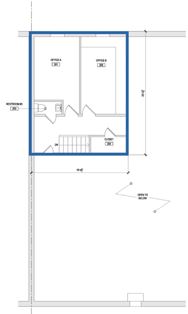
SECOND FLOOR
