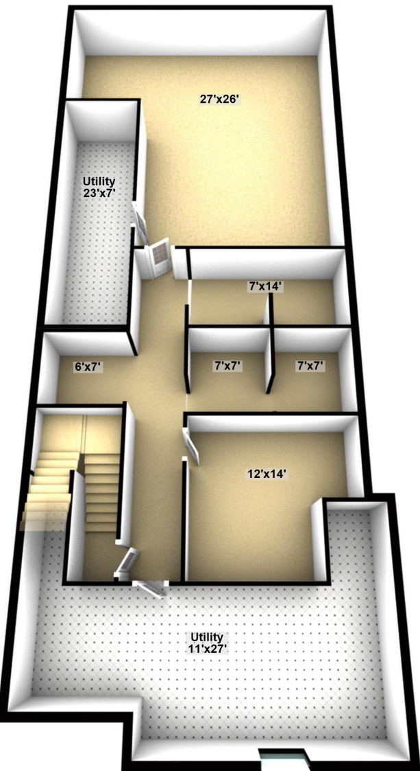
Lower Level
