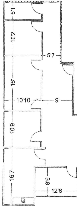
LAYOUT B 1,107 SF
