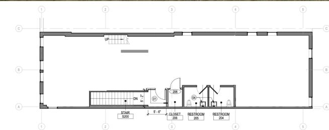
3 FLOOR PLAN - LEVEL 2 1/8" = 1'-0"
